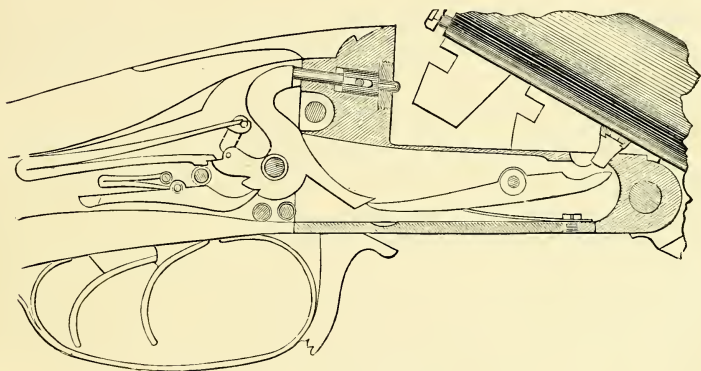
Hill's Hammerless Gun.
